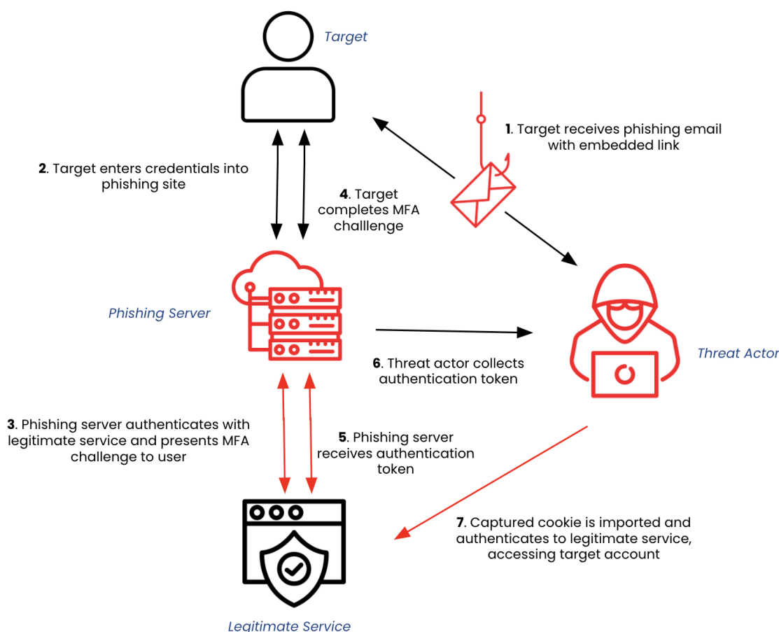
High-level example of how a token theft attack can take place
